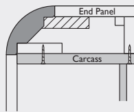
Step 2 - Fix to Carcass
