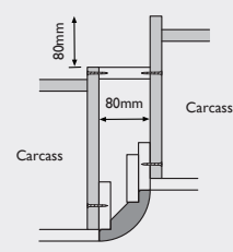
Step 2 - Fix to Carcass
