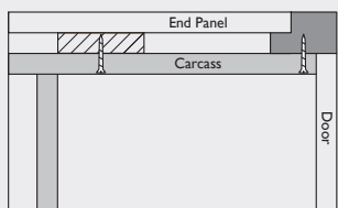
Step 2 - Fix to Carcass
